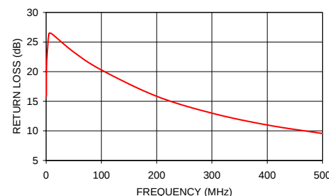
ADT4-5WT INPUT RETURN LOSS
