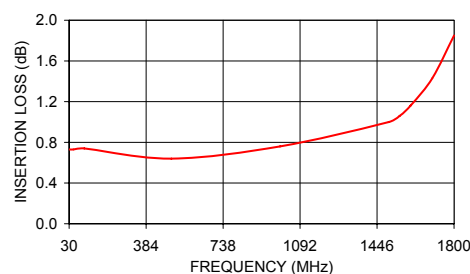
ADTL2-18 INSERTION LOSS
