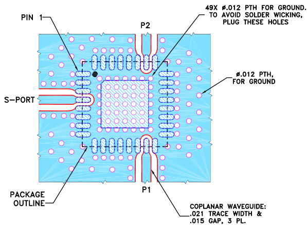
Demo Board MCL P/N: TB-880W+ Suggested PCB Layout (PL-488)
