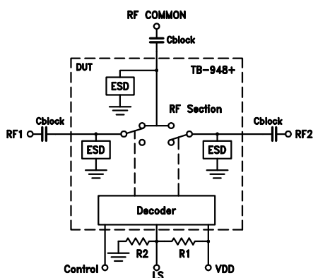
Figure 1. Block Diagram of test Circuit used for characterization (DUT, R1&R2 soldered on Mini-Circuit's TB-948+) R1=2.21k \Omega R2=3.32k \Omega
