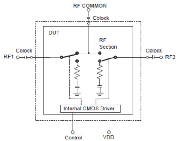
Figure 1. Block Diagram of test Circuit used for characterization (DUT soldered on Mini-Circuit's TB-159A+)
