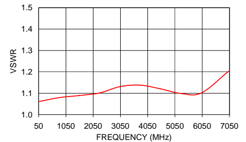
PAT-4+ VSWR
