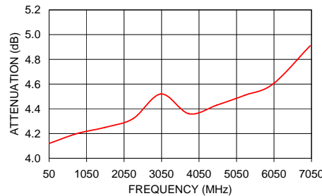
PAT-4+ ATTENUATION
