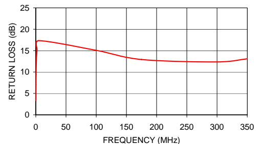
T4-1-KK81 INPUT RETURN LOSS
