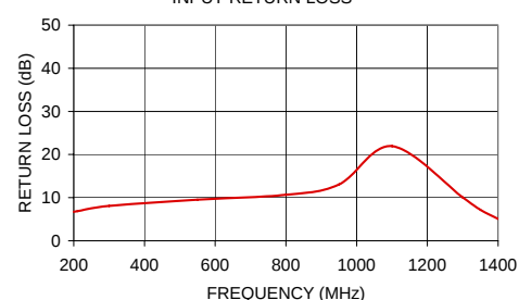
TC4-14G2+ INPUT RETURN LOSS
