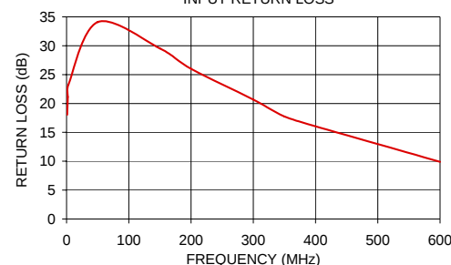
TC4-6TG2+ INPUT RETURN LOSS
